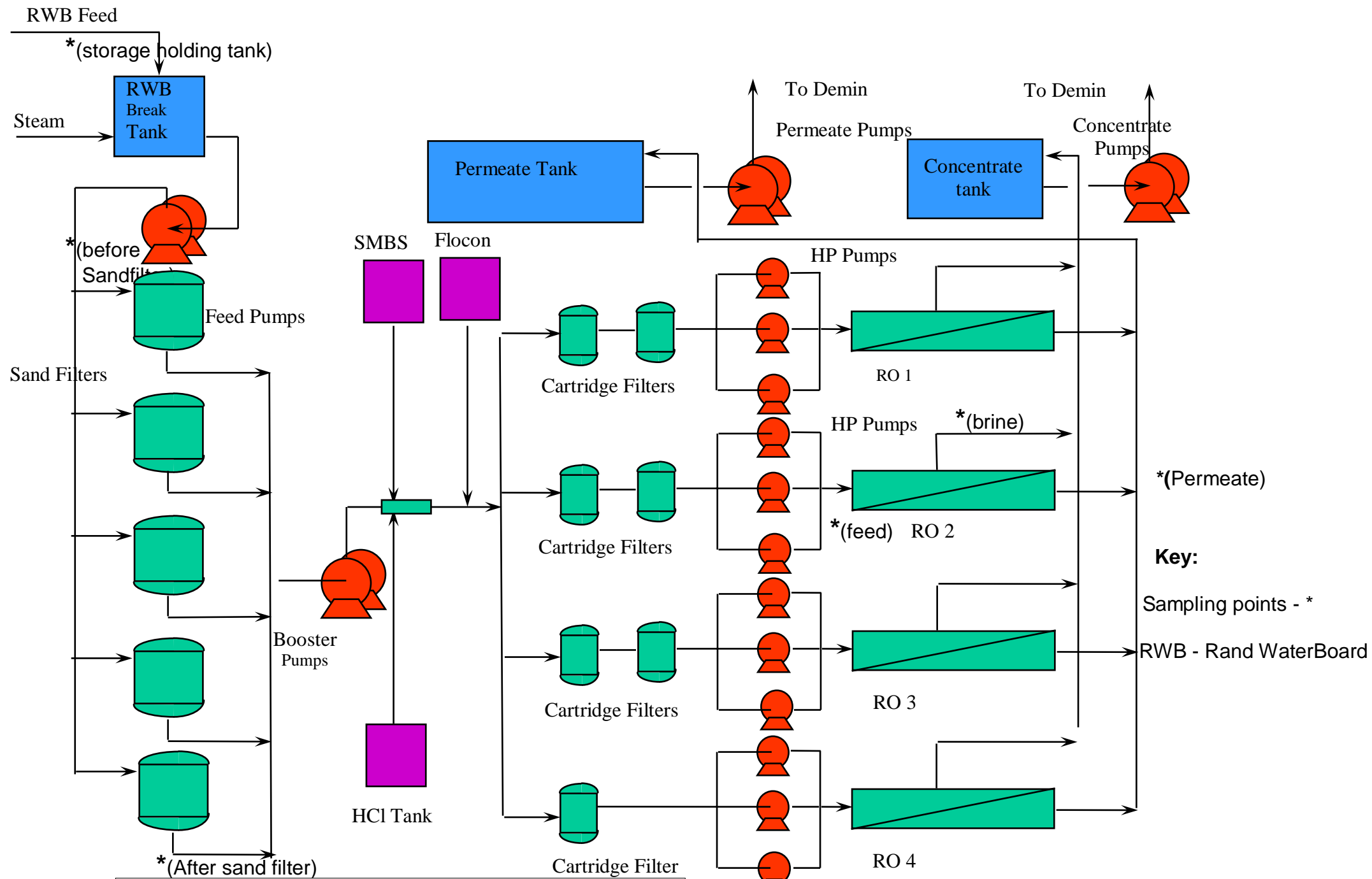
Figure 3.3 RO Plant simplified flow diagram
